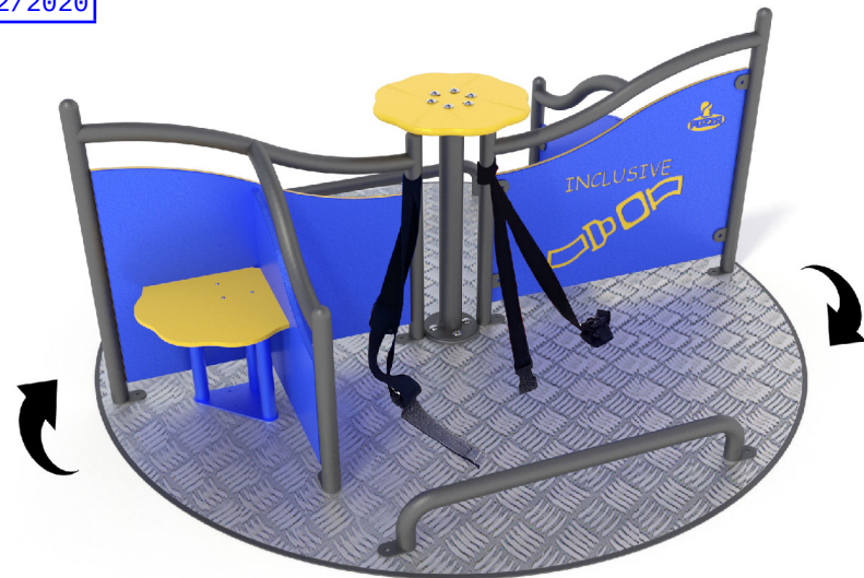
A G0300H1 GIOSTRA GIROTONDO INCLUSIVE Safety area: 5.8x5.8m
